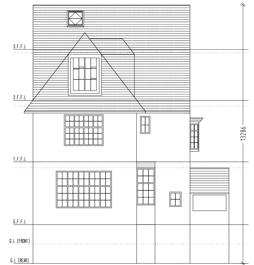
REAR ELEVATION
