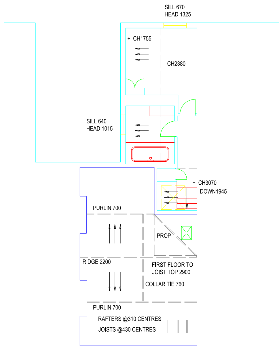
SECOND FLOOR / LOFT SPACE
