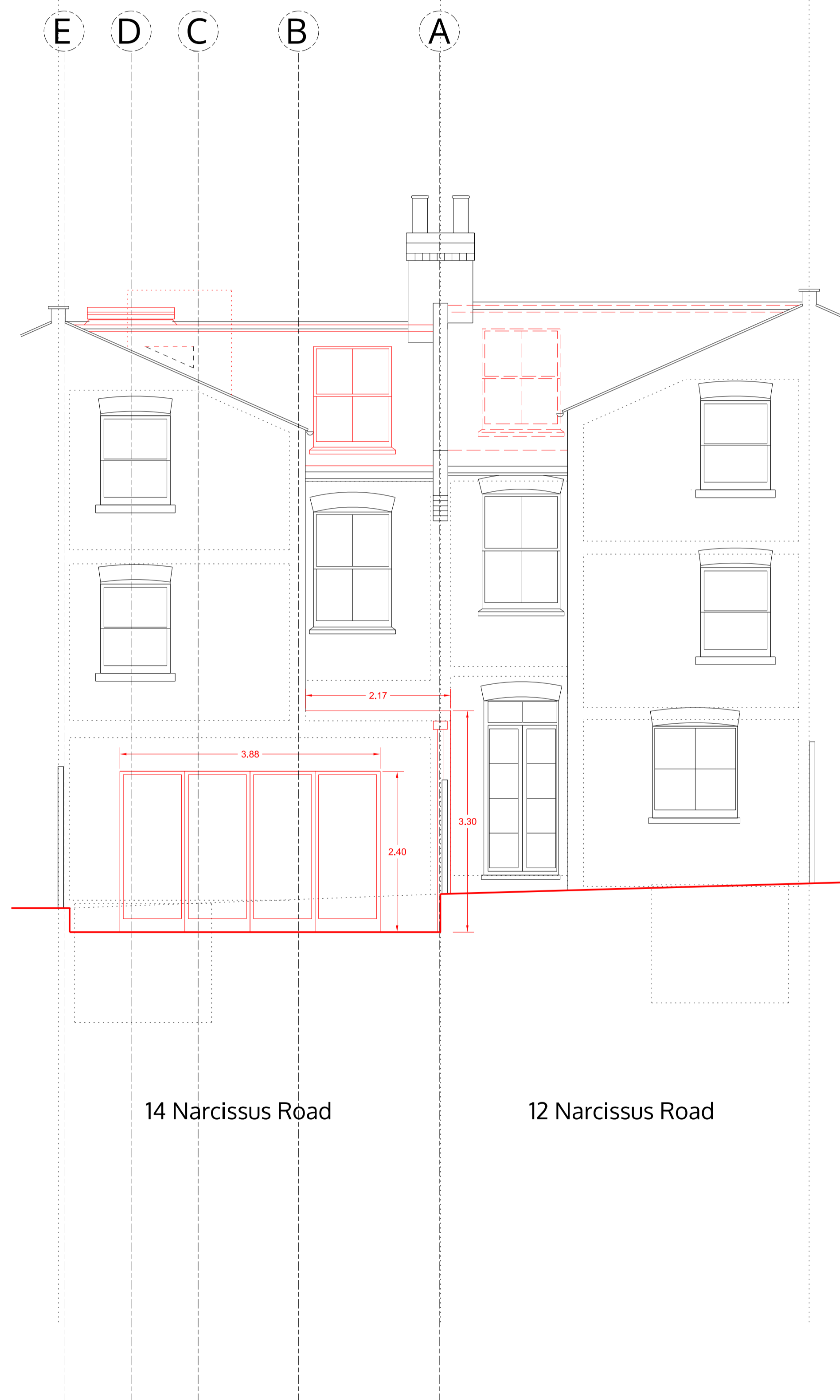
Rear elevation
