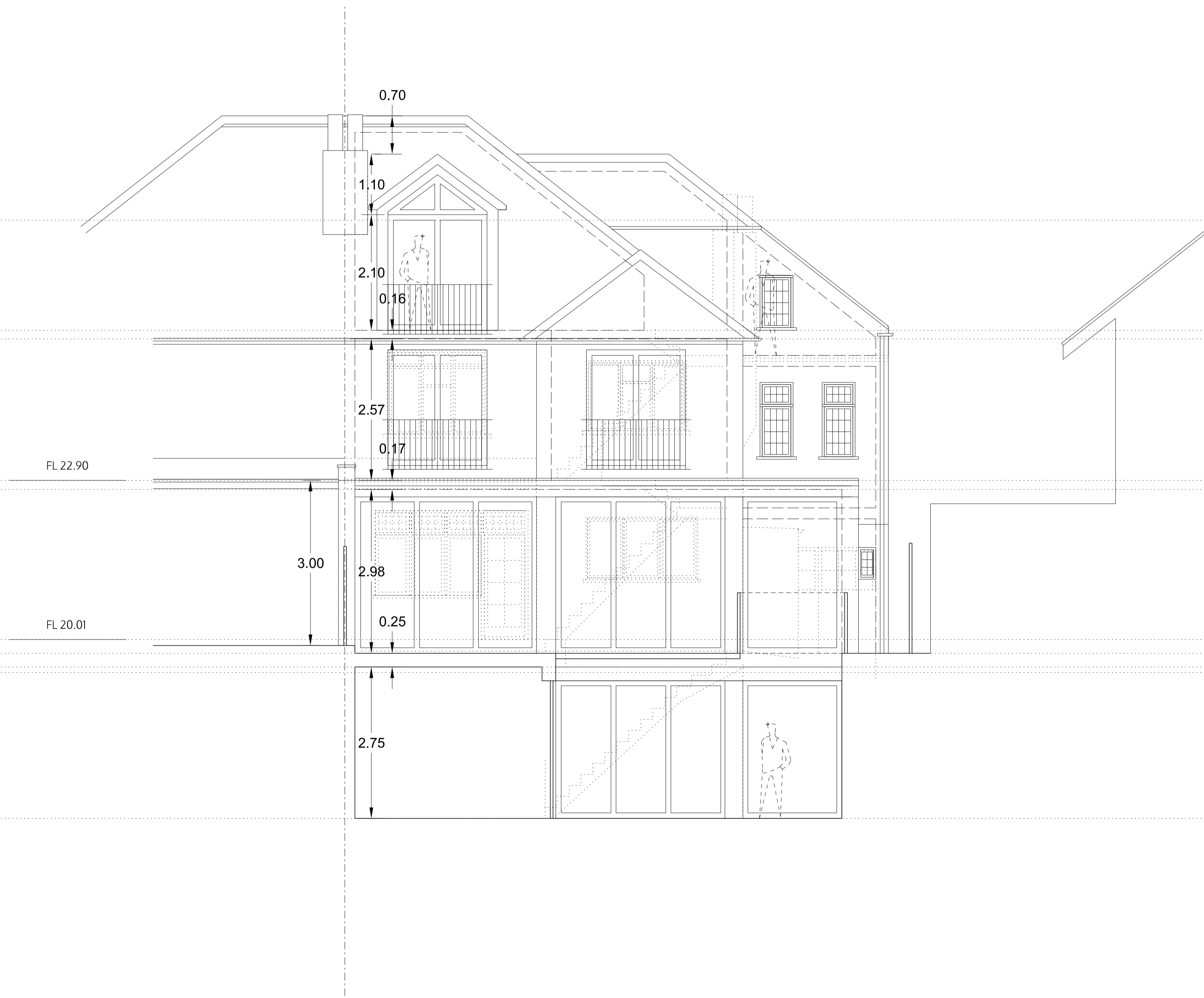
REAR ELEVATION (WEST)
