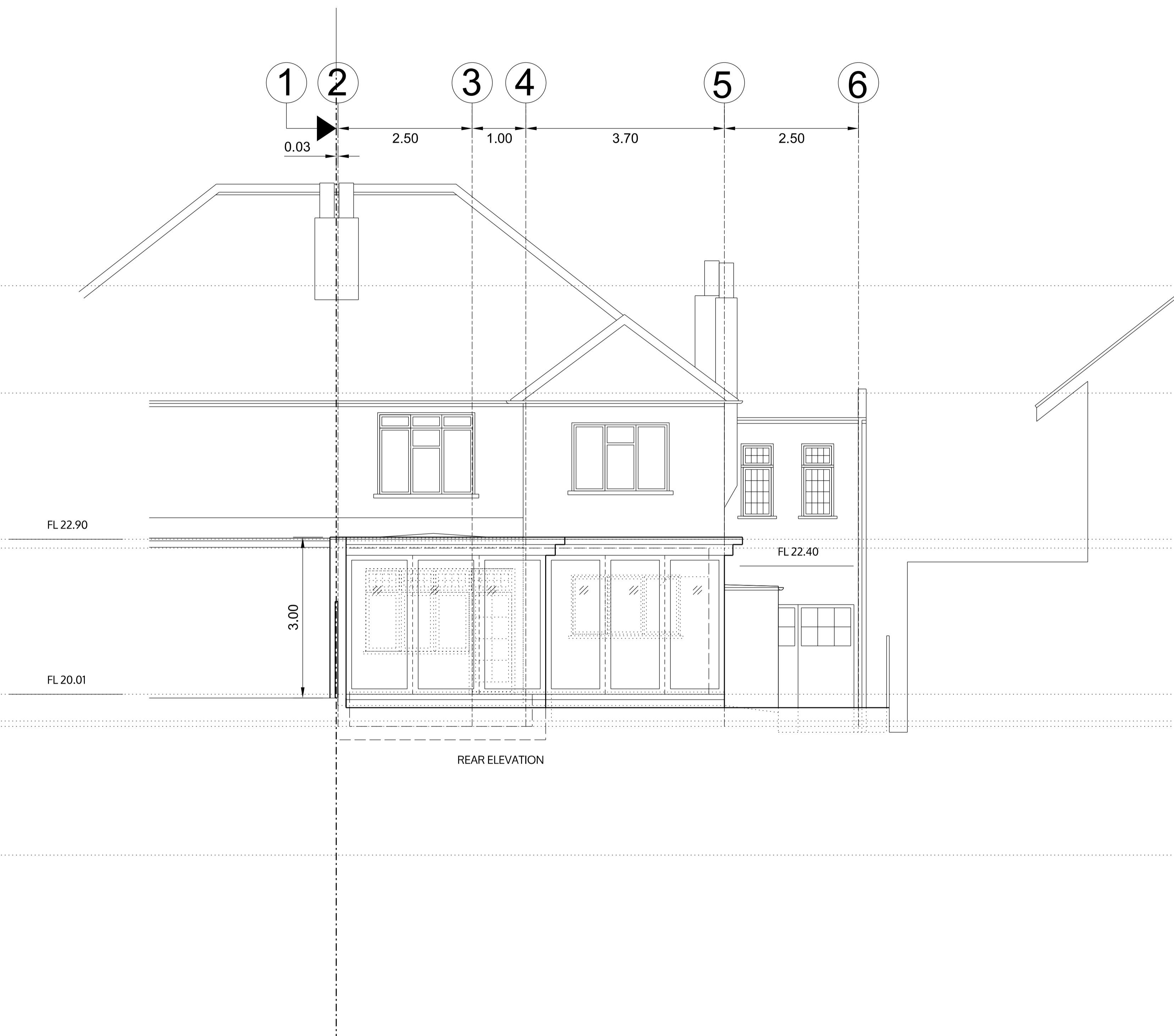
REAR ELEVATION (WEST)
