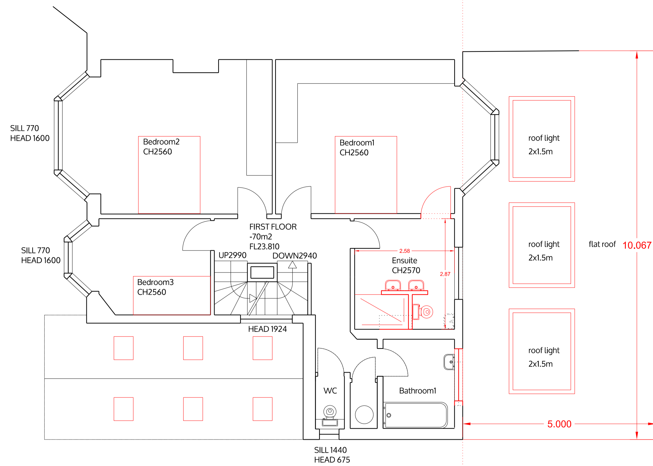
FIRST FLOOR
