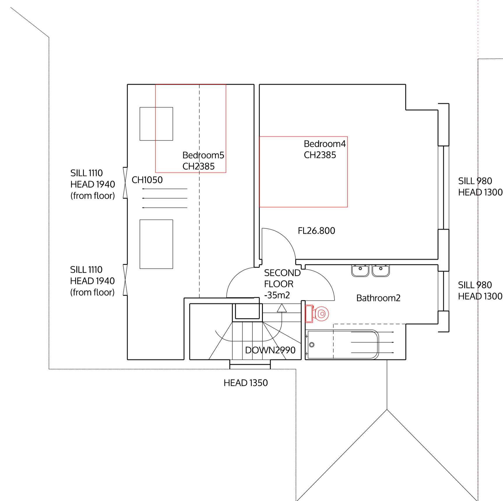
SECOND FLOOR
