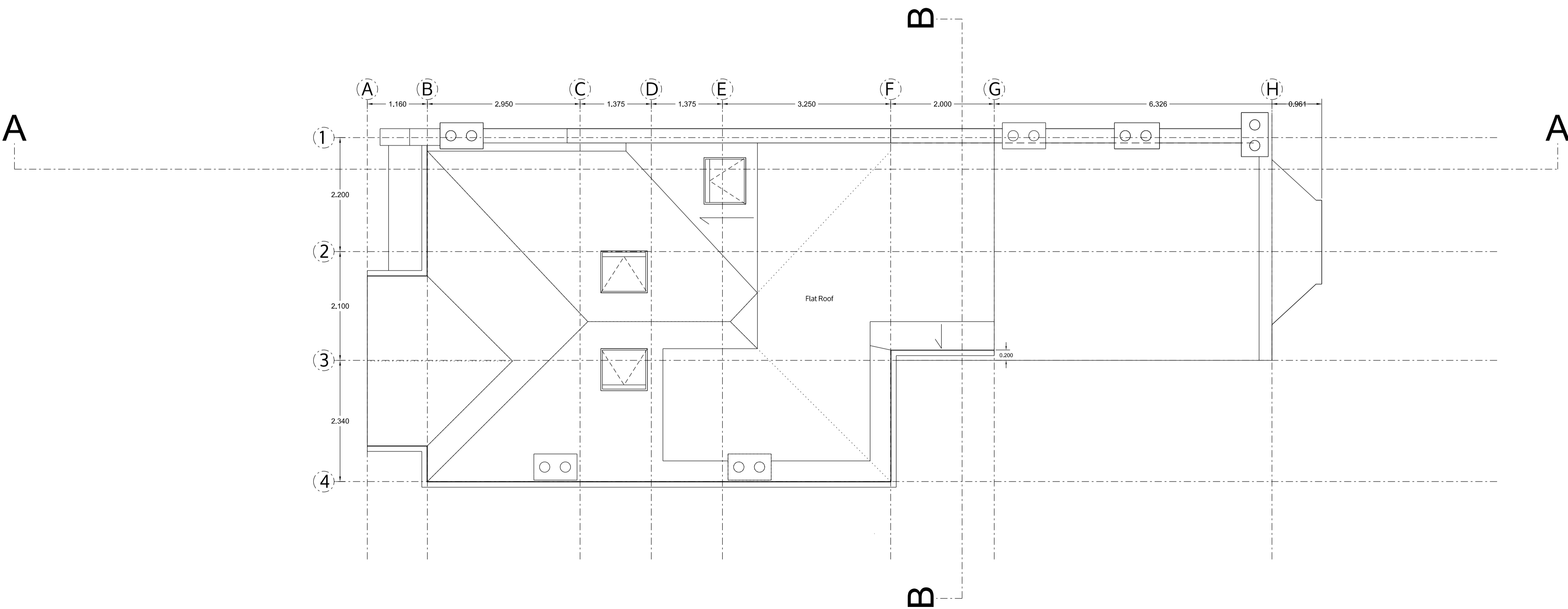
ROOF PLAN
