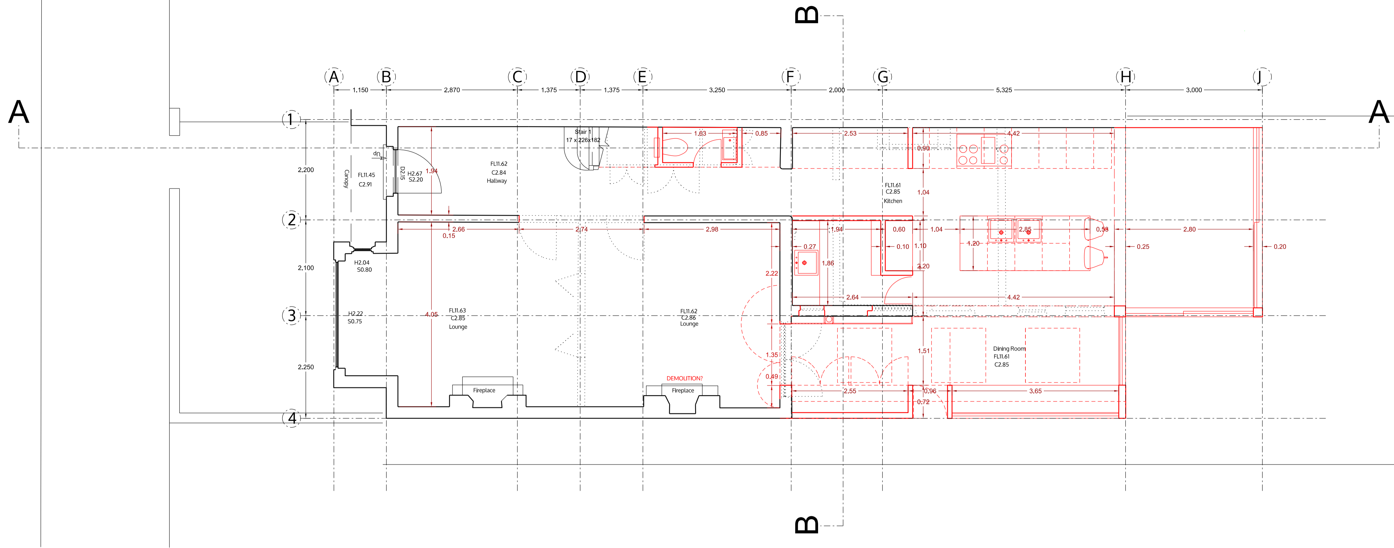
GROUND FLOOR
