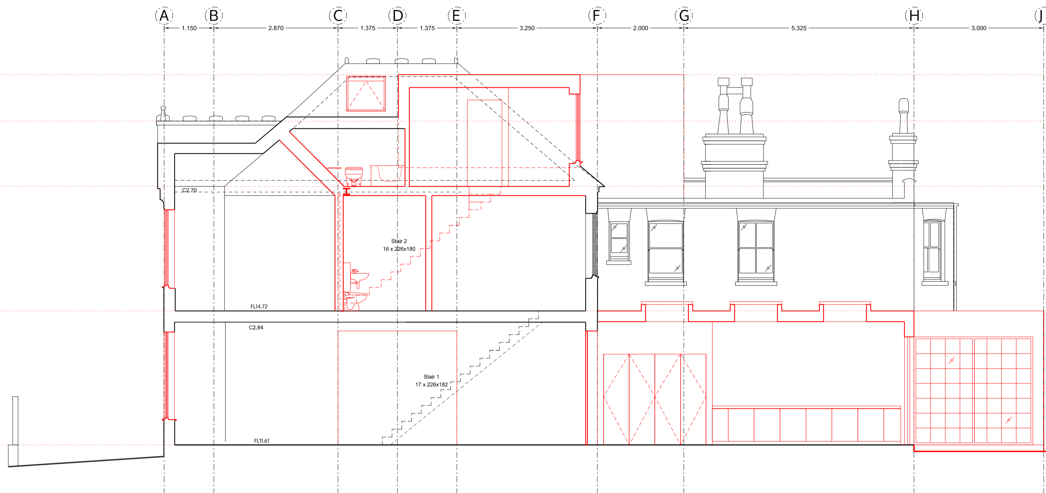
SECTION BB
