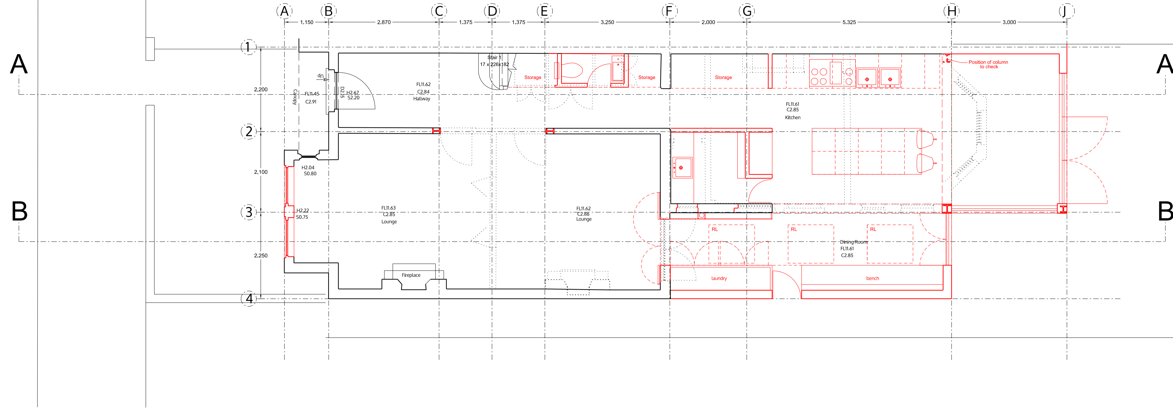
GROUND FLOOR
