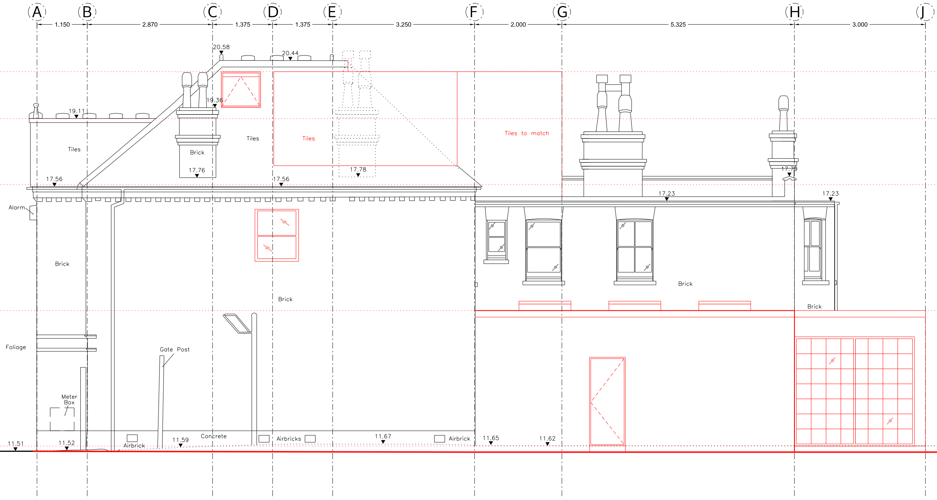
SIDE ELEVATION
