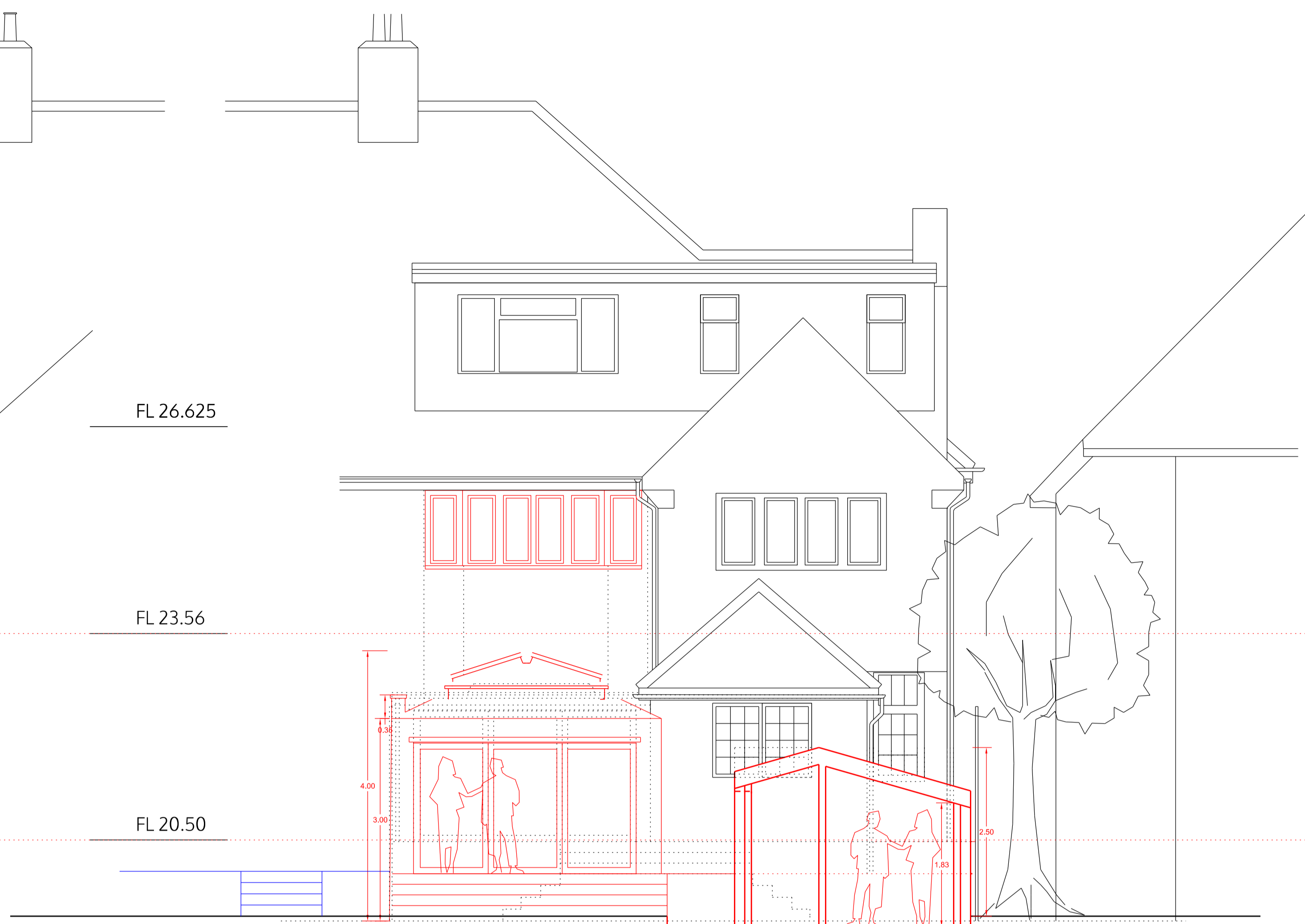
REAR ELEVATION
