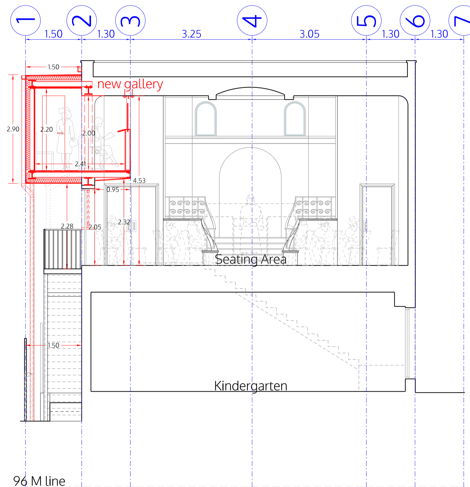
Section B-B
