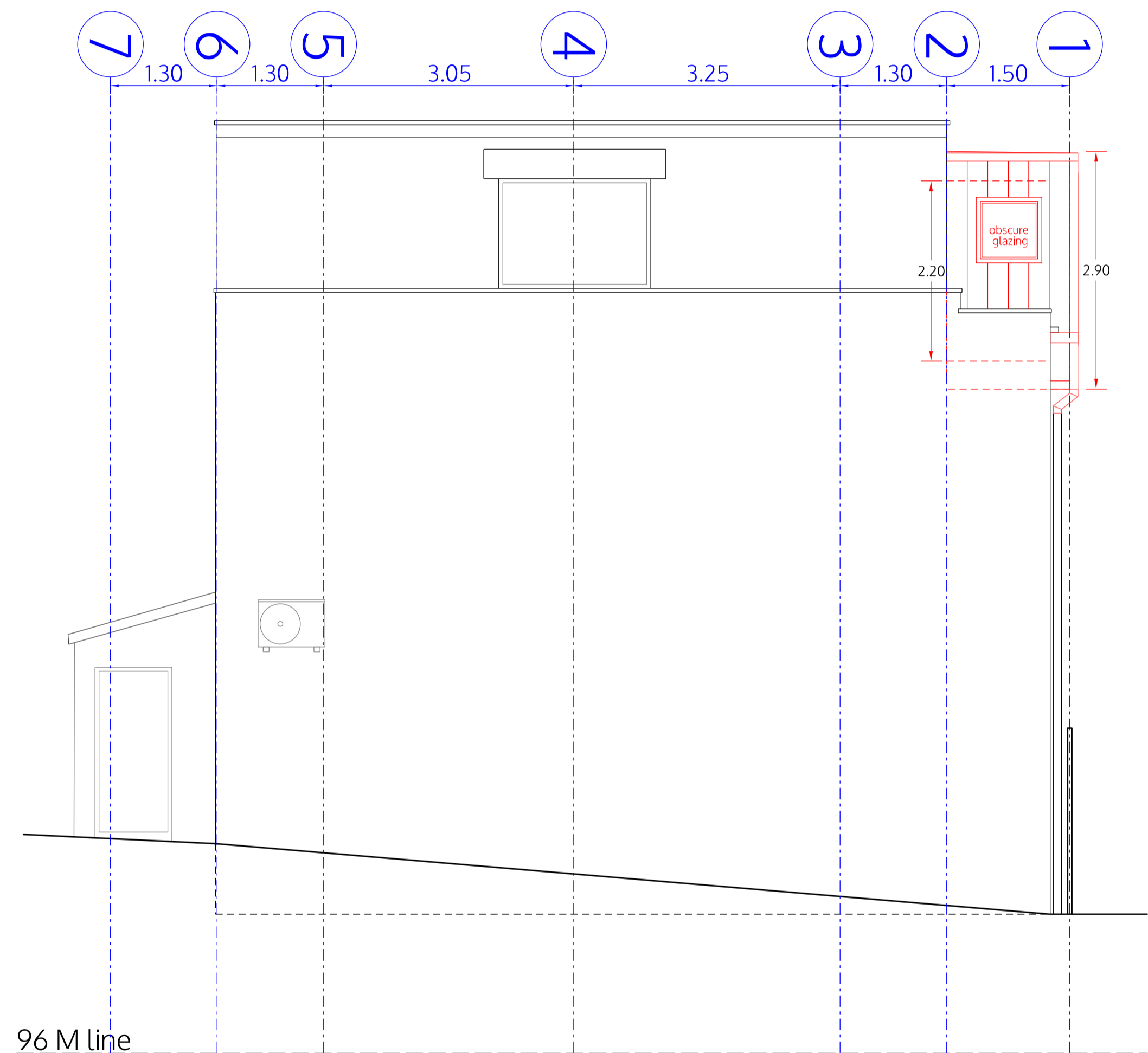
Southeast elevation
